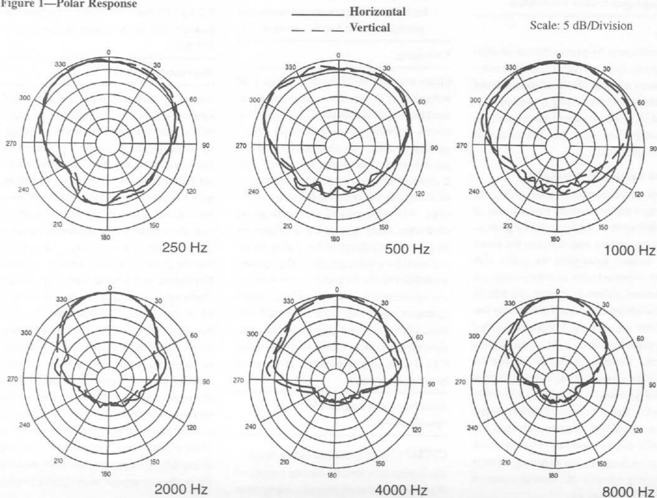
Figure 1—Polar Response
